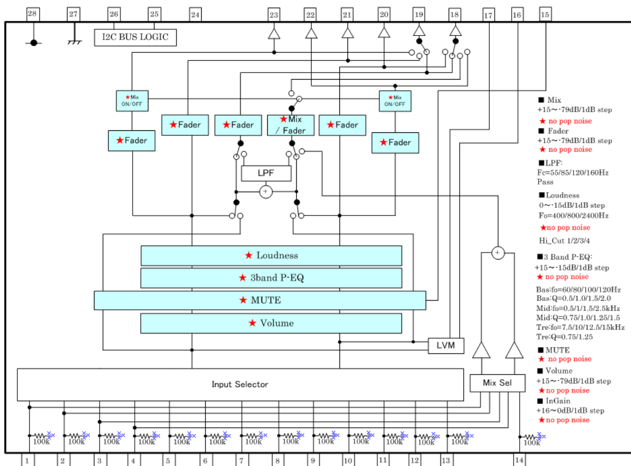
Figure 3. Block Diagram
