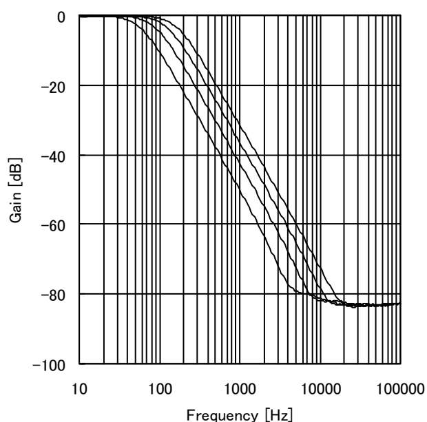
Figure 15. LPF
