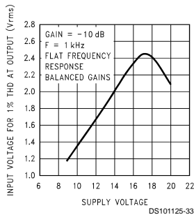
Input Signal Handling vs Supply Voltage
