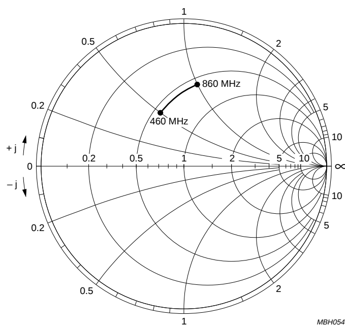
Fig.14 Input impedance ( S_{11} ) of the band C mixer input (460 to 860 MHz); Z_0 = 50 \Omega .
