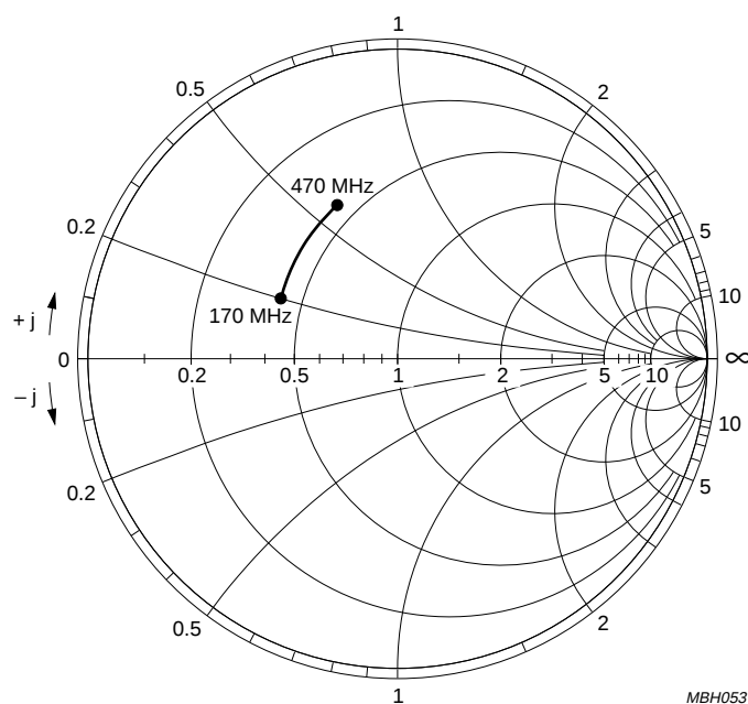
Fig.13 Input impedance ( S_{11} ) of the band B mixer input (170 to 470 MHz); Z_0 = 50 \Omega .
