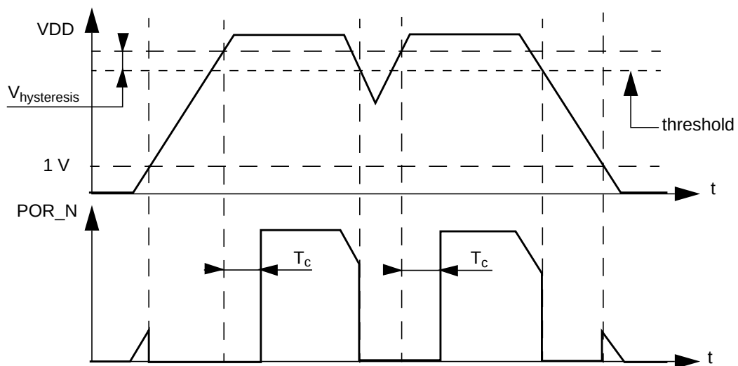
Fig.21 Power on reset timing
