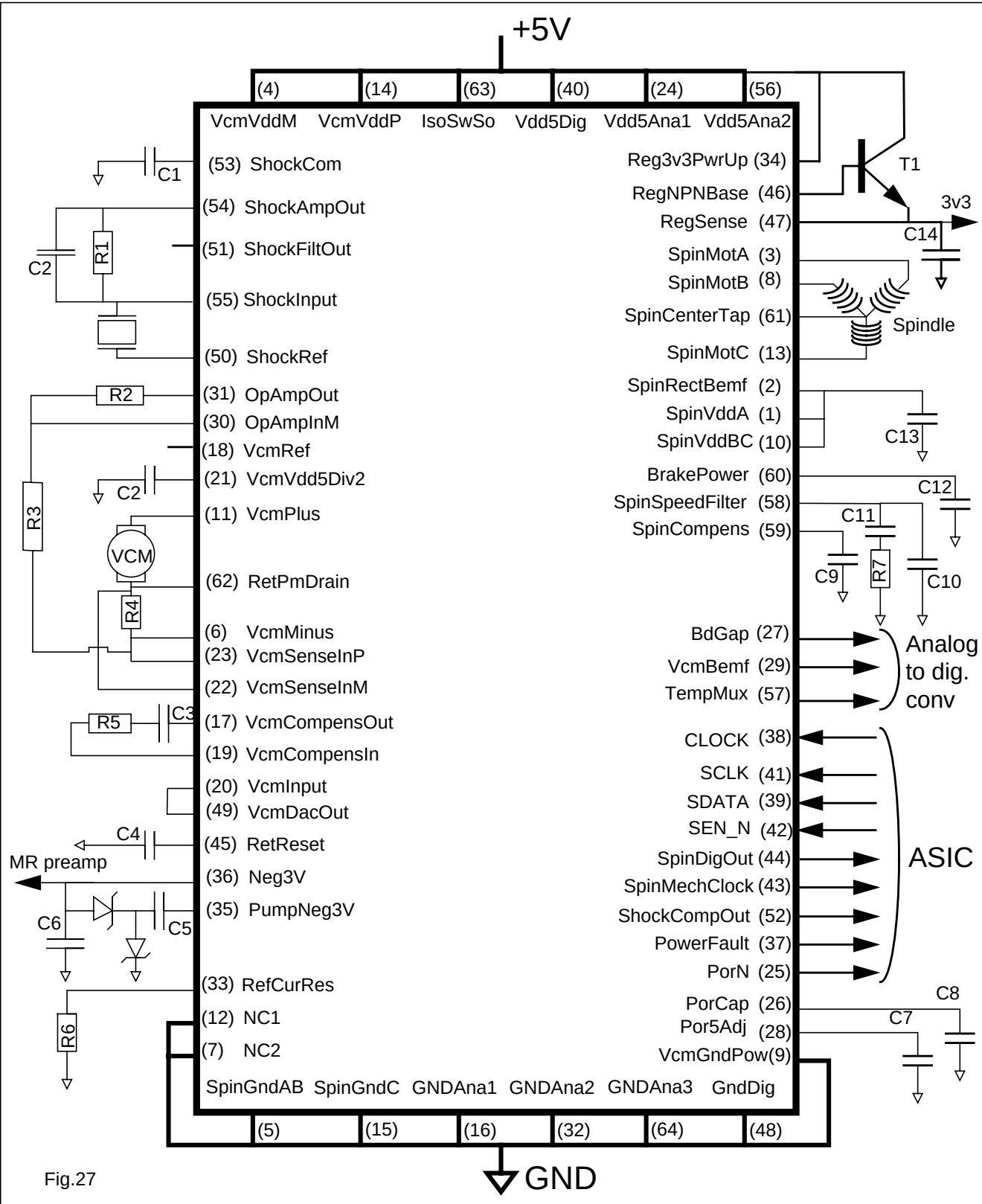
TYPICAL APPLICATION SCHEMATIC
