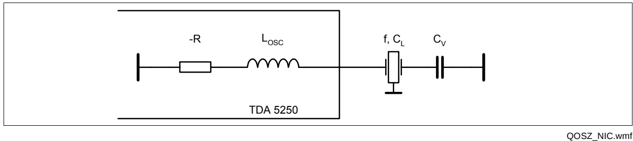
Figure 3-13 Crystal Oscillator
