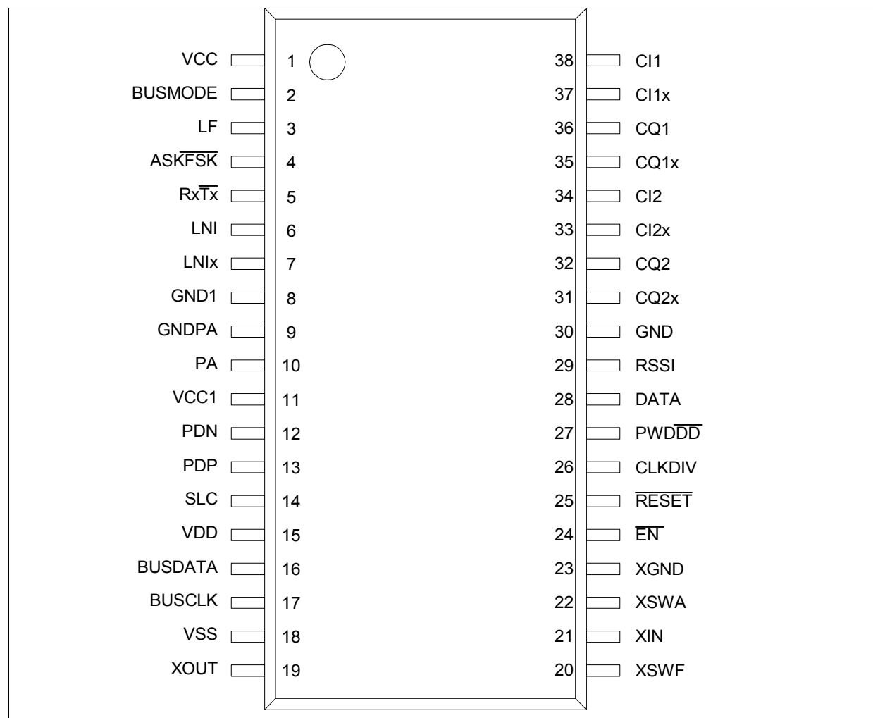
Figure 2-1 Pin Configuration
