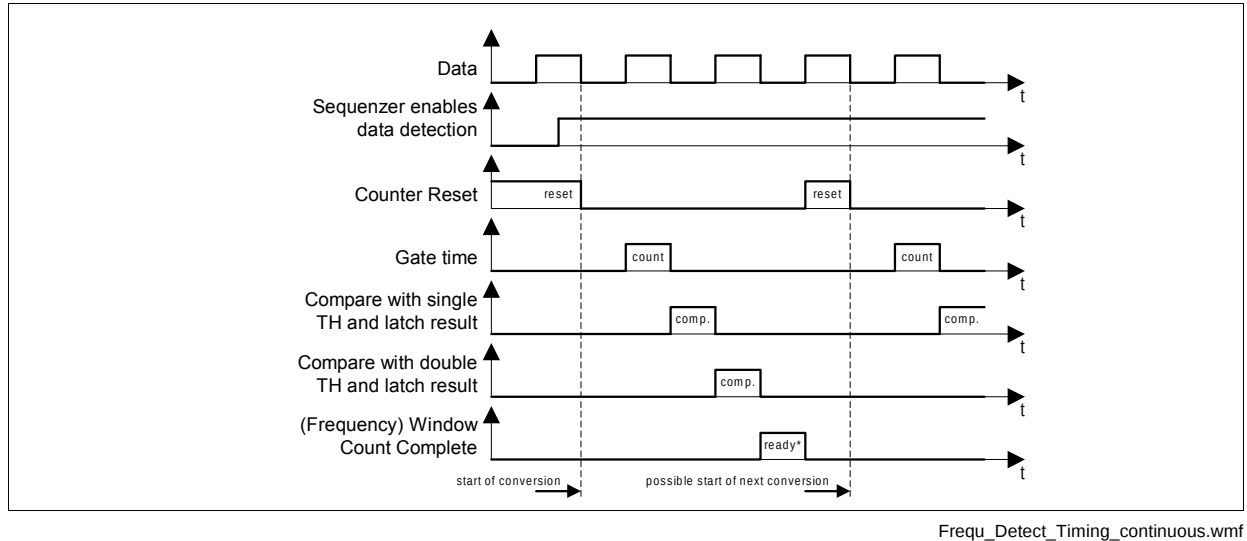
Figure 3-29 Frequency Detection timing in continuous mode
