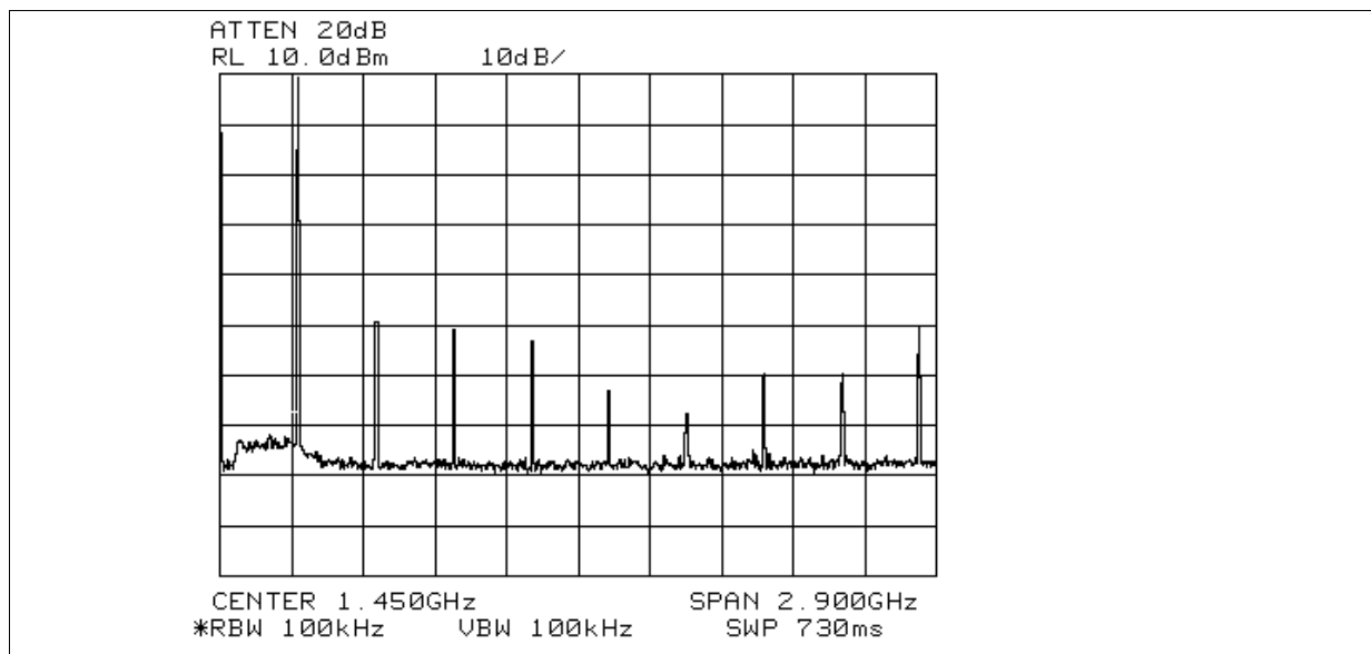
Figure 3-10 Transmit Spectrum 3GHz
