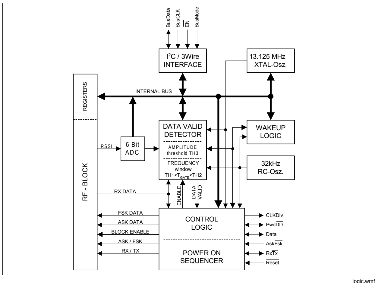
Figure 2-6 Timing and Data Control Unit
