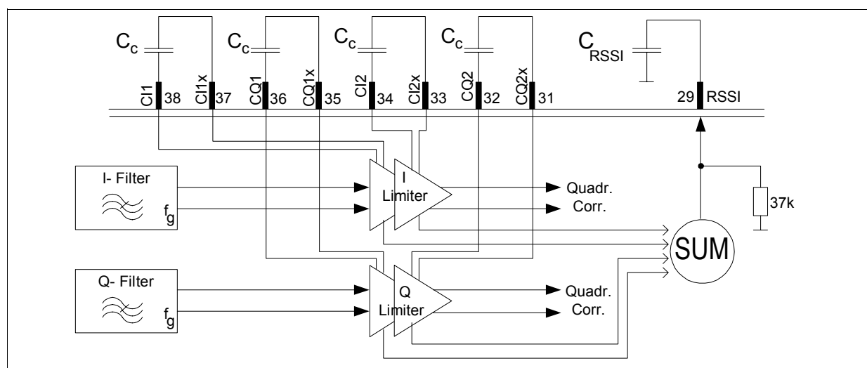
Figure 3-20 Limiter and Pinning
