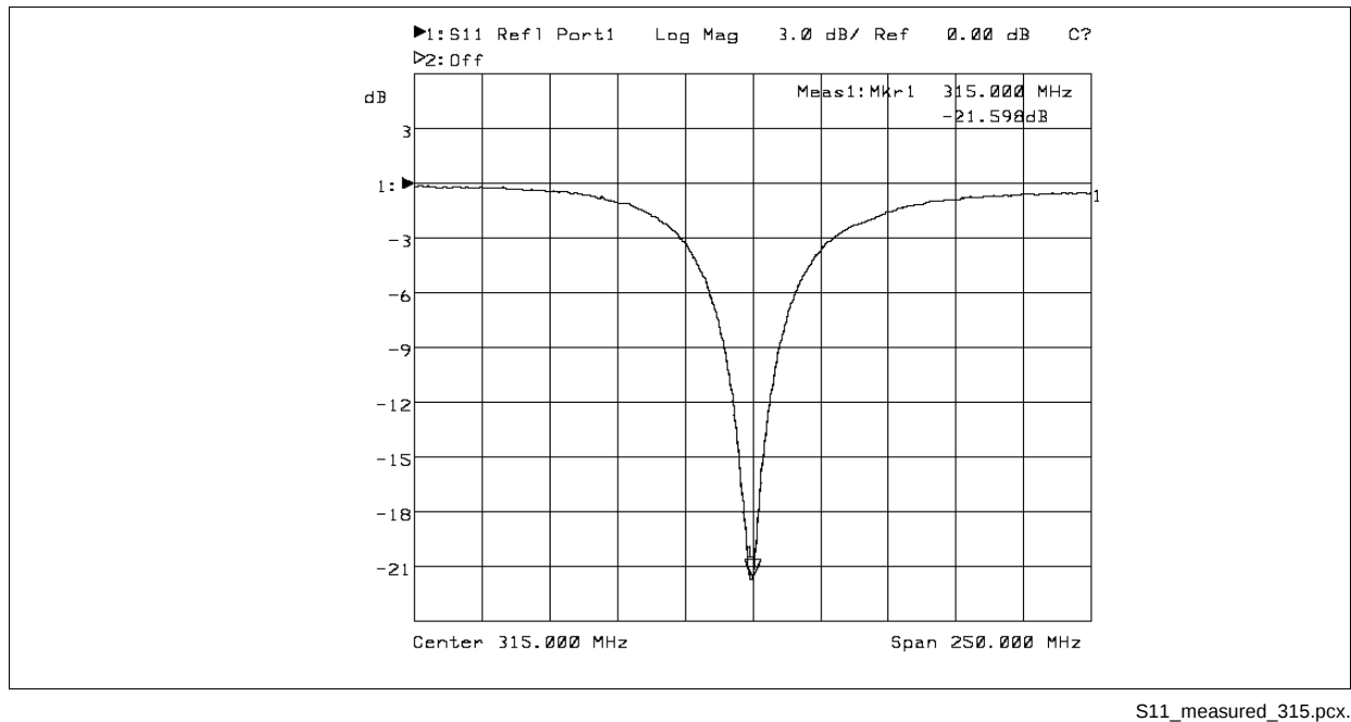
Figure 3-3 S11 measured
