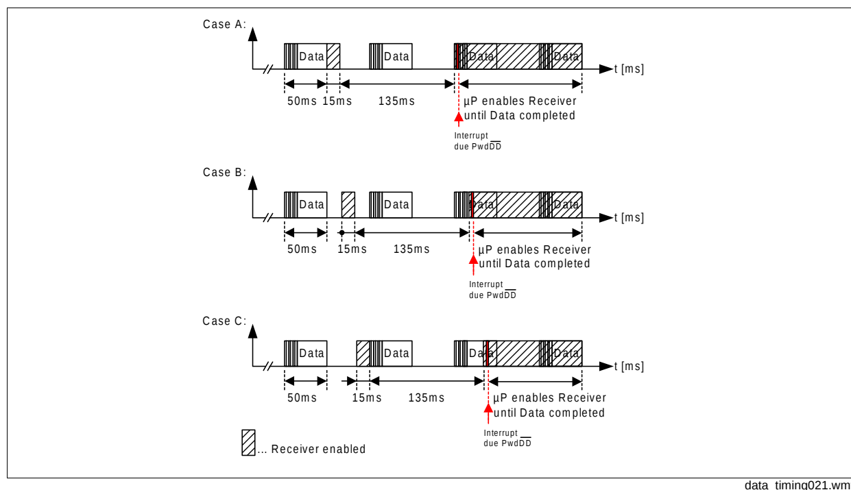
Figure 3-33 3 possible timings
