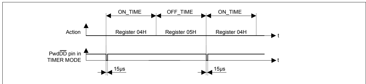
Figure 2-11 Timing for Timer Mode
