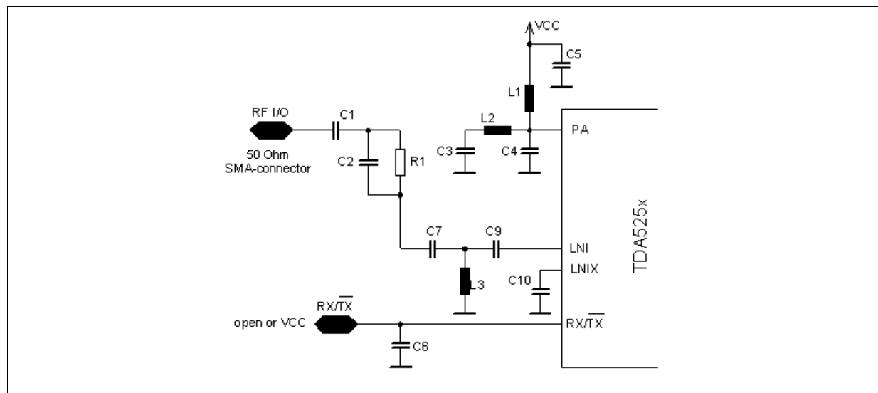
Figure 3-2 RX-Mode
