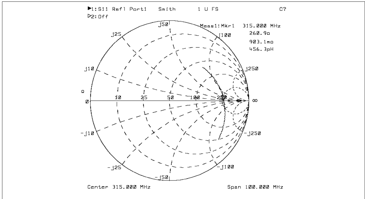
Figure 3-9 Sparam_measured_100M
