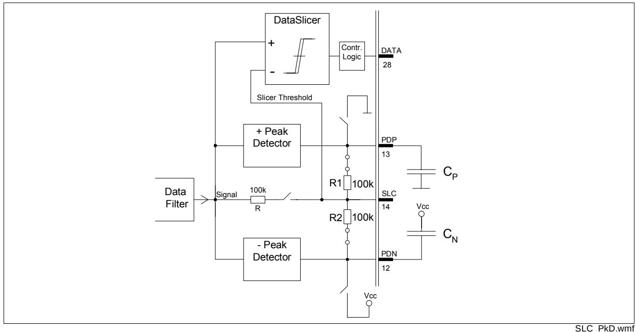
Figure 3-24 Slicer Level using Peak Detector
