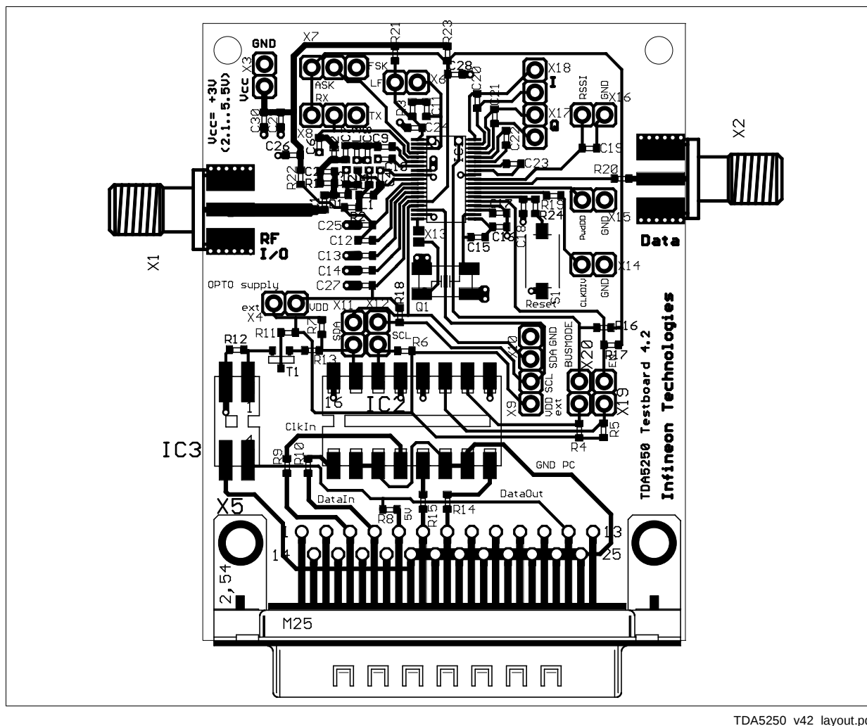
Figure 4-4 Layout of the Evaluation Board
