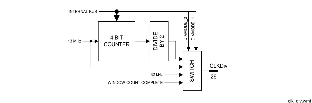
Figure 2-18 Clock Divider
