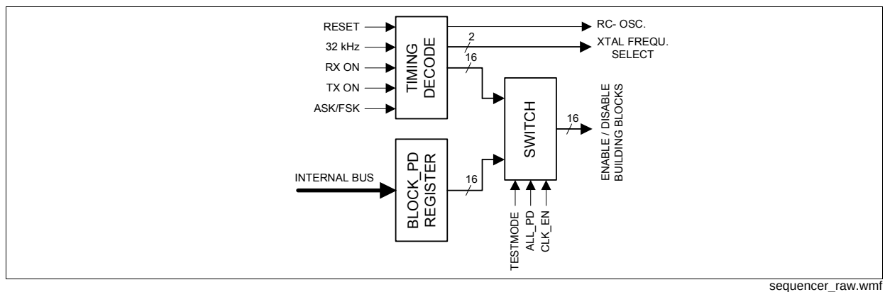
Figure 2-17 Sequencer's capability
