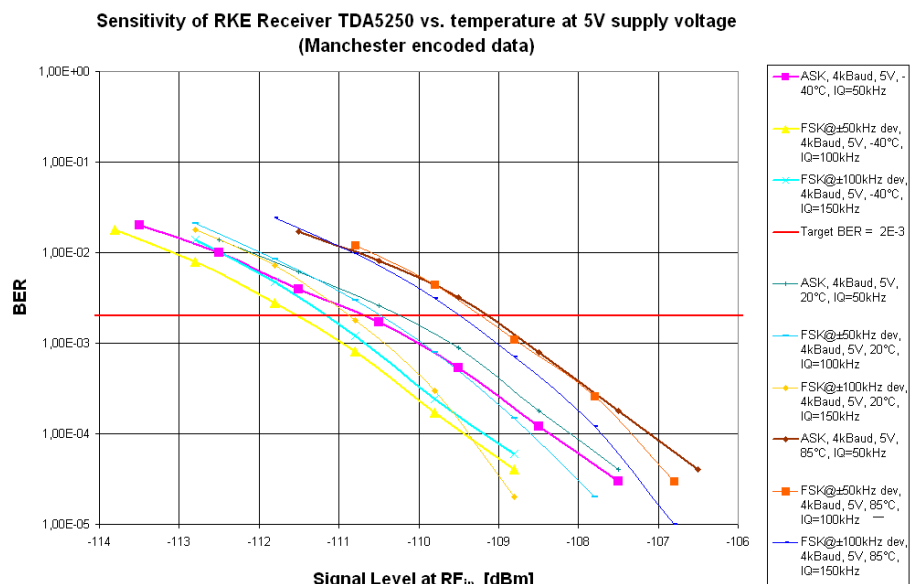
Figure 4-37 Temperature Behaviour
