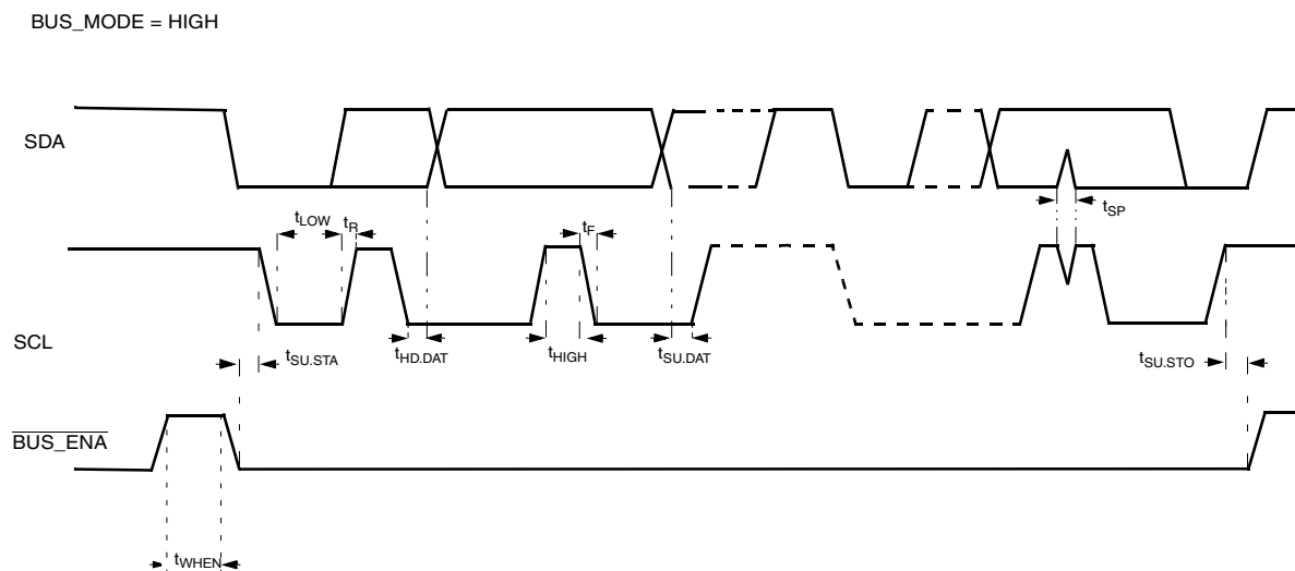
Figure 5-2 3-wire Bus Timing
