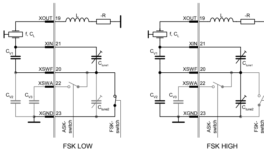
Figure 4-17 FSK modulation
