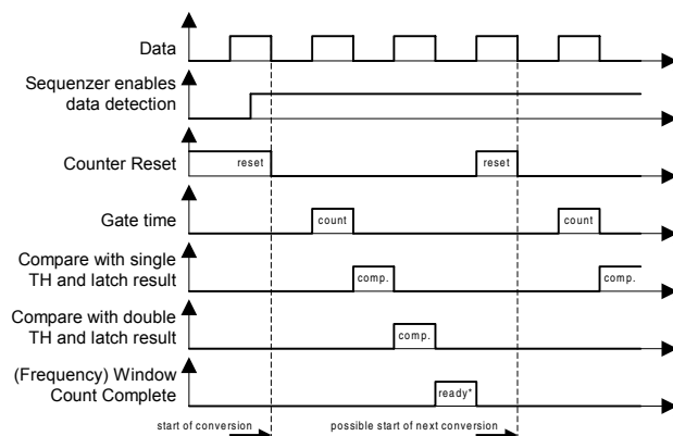
Figure 4-31 Frequency Detection timing in continuous mode
