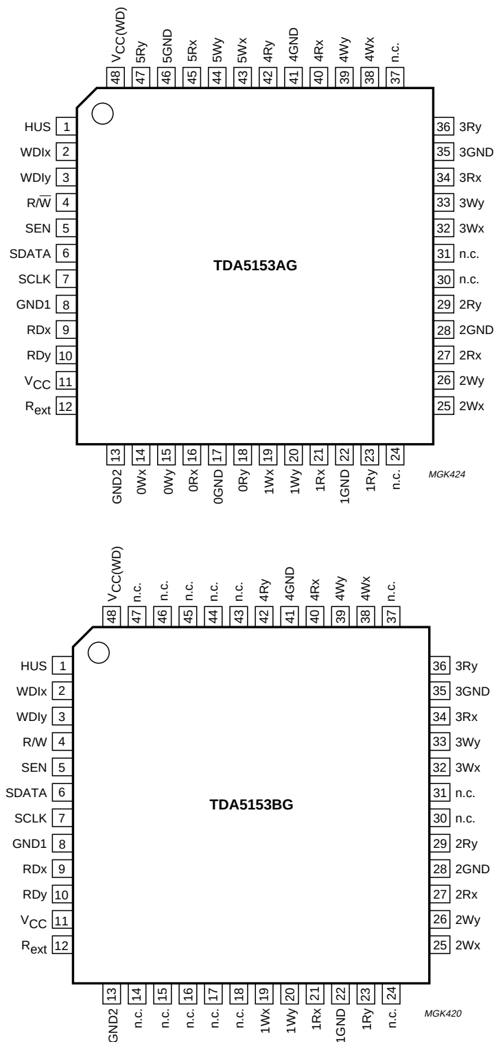
Fig.2 Pin configurations.
