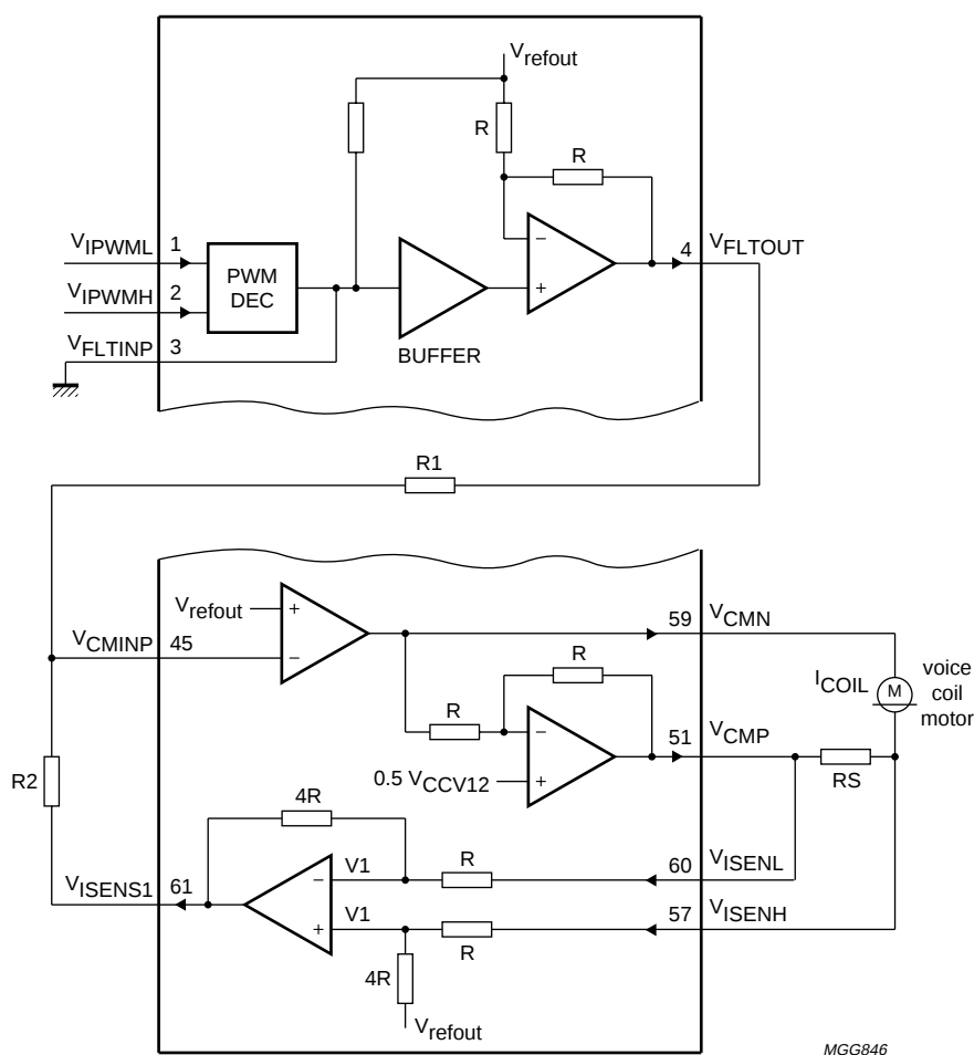
Fig.4 Transconductance model.
