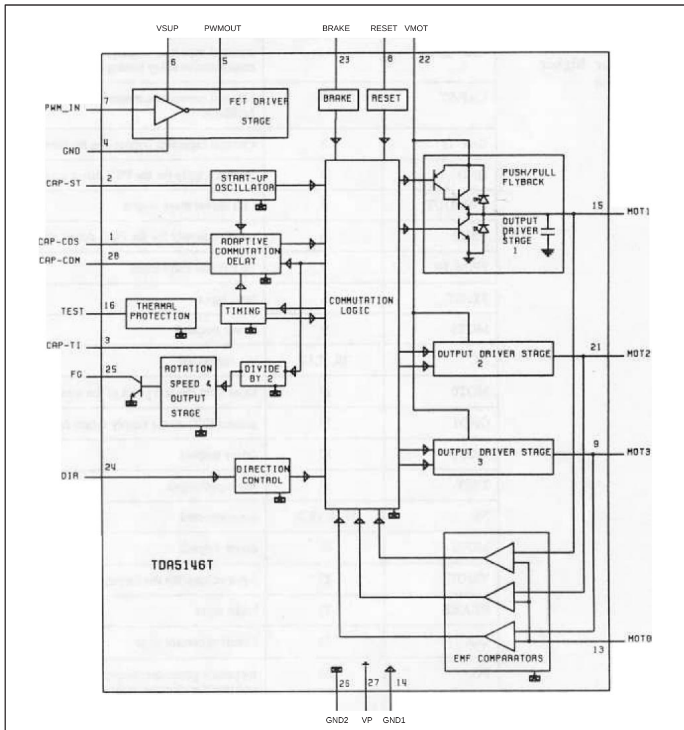
Figure 1. Block diagram
