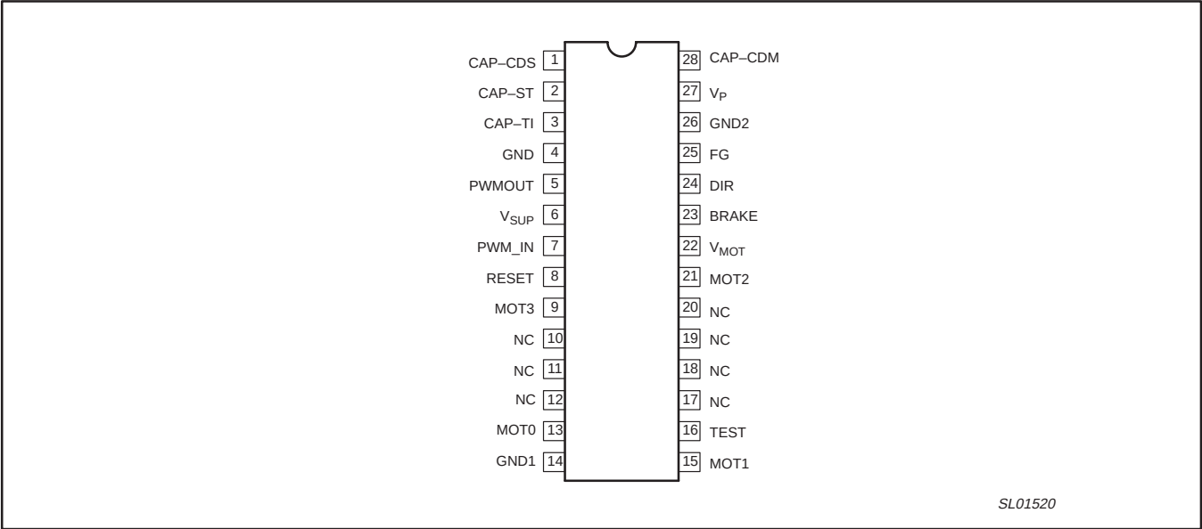
Figure 2. Pin configuration
