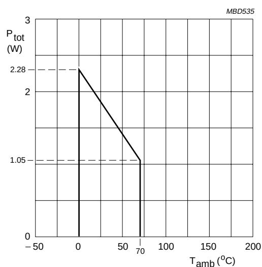
Fig.4 Power derating curve (SOT102; DIL18).
