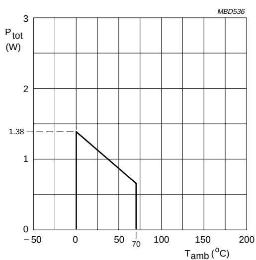
Fig.5 Power derating curve (SOT163A; SO20L).
