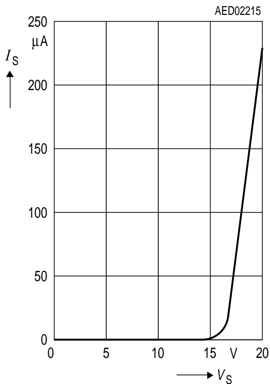
Quiescent Current I_S versus Supply Voltage V_S ; inhibit mode; T_j = 25^\circ\text{C}
