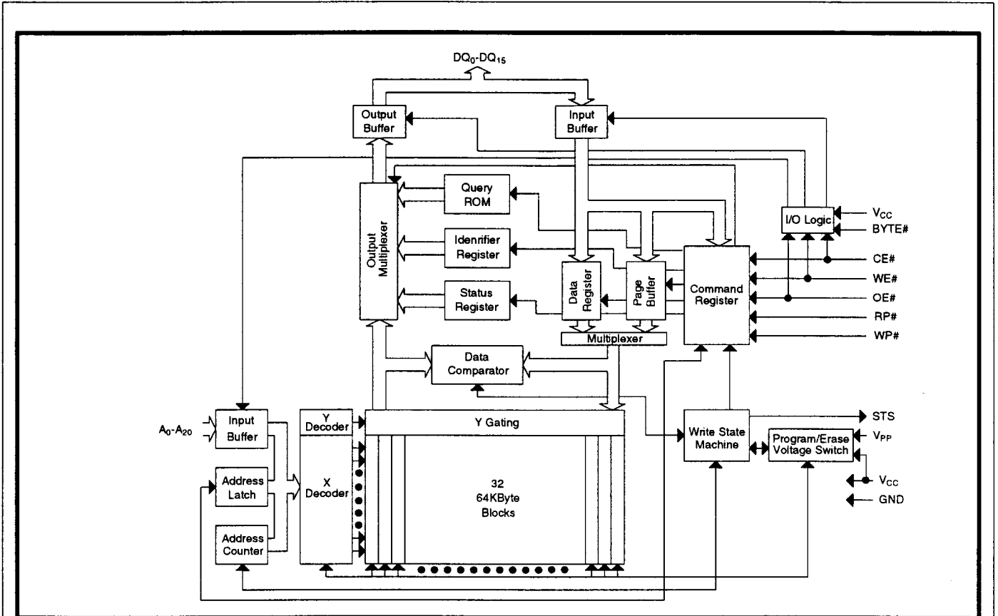
Figure 1. Block Diagram
