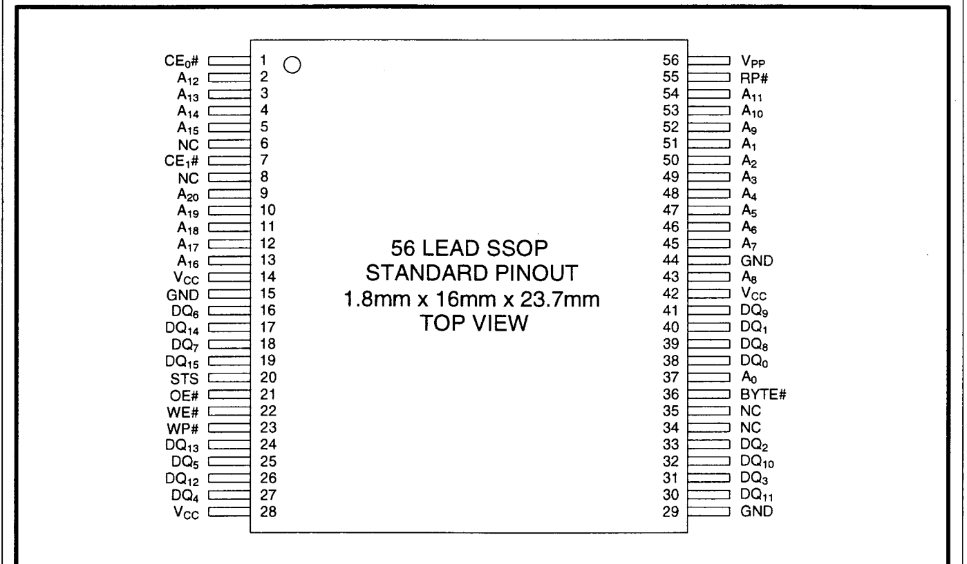
Figure 2. SSOP 56-Lead Pinout
