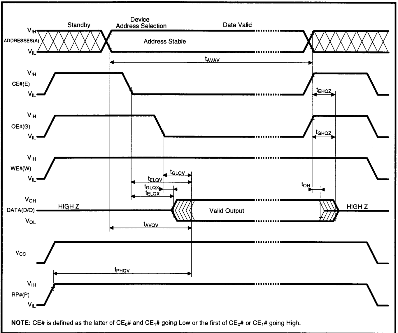
Figure 17. AC Waveform for Read Operations
