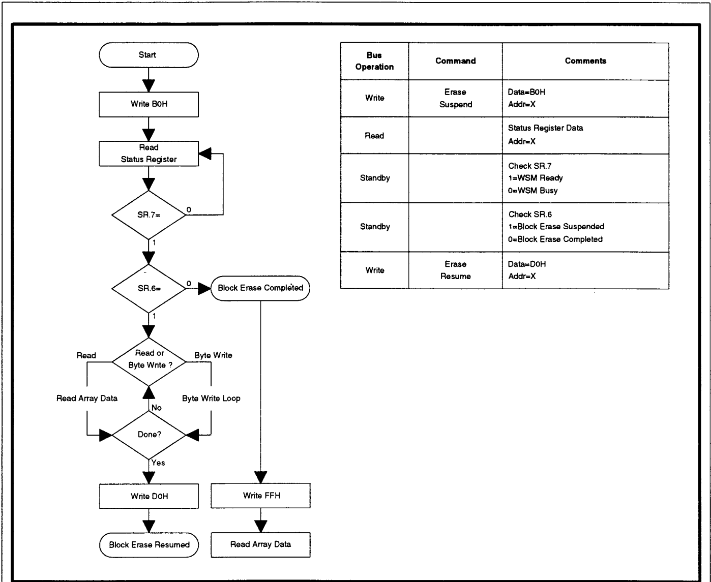
Figure 7. Block Erase Suspend/Resume Flowchart
