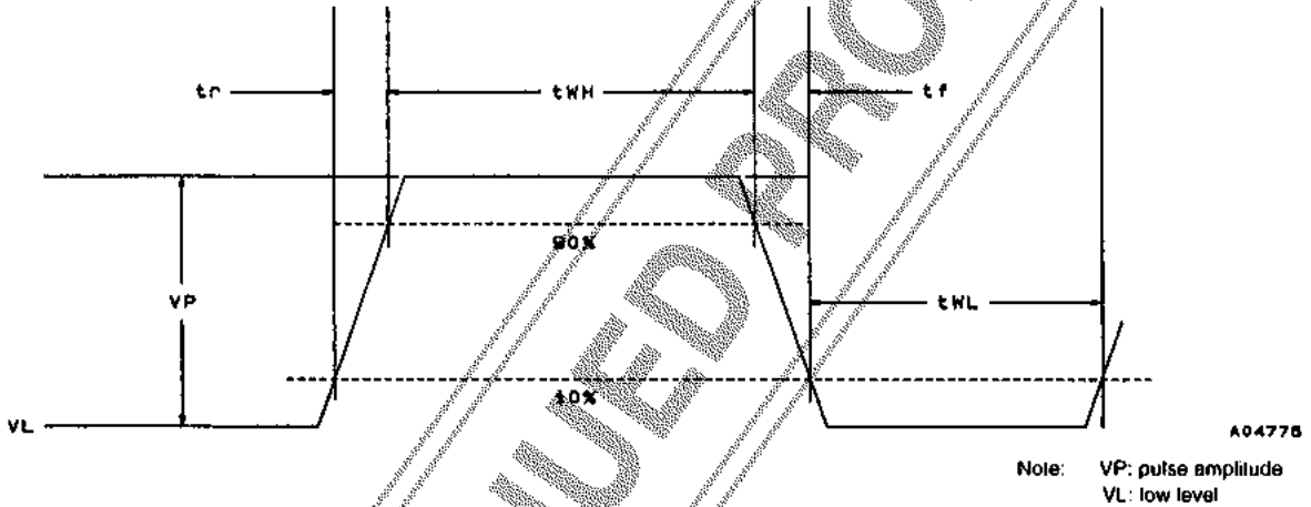
Figure 3 Pulse Waveform
