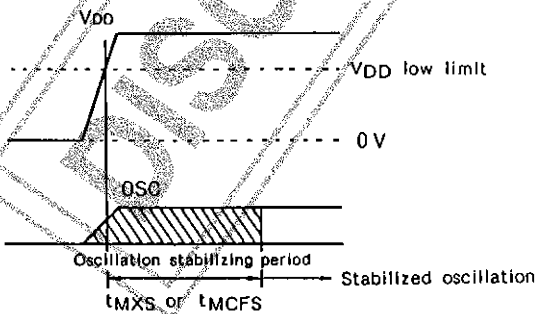
Fig. 2. Main clock oscillation stabilizing period
