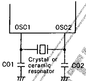
Fig. 1 Main clock oscillation circuit
