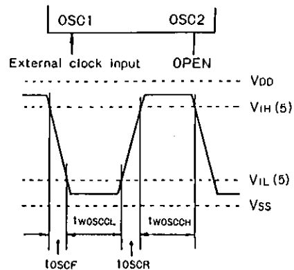
Fig.3. Input waveform of input clock (for main clock)
