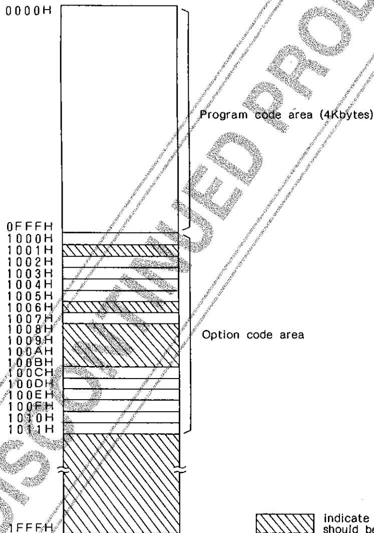
EPROM address map
