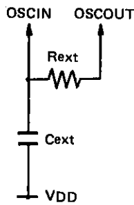
Fig. 12 RC oscillation
