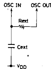
Fig.8 Recommended CR oscillation circuit
