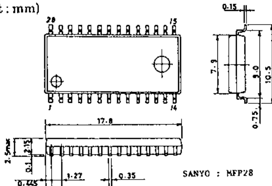
Case Outline 3091-M28IC (unit : mm)
